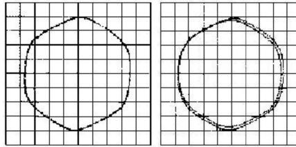
Figure 1: Parks vector for a healthy motor (left) and a motor with air-gap eccentricity (right)
